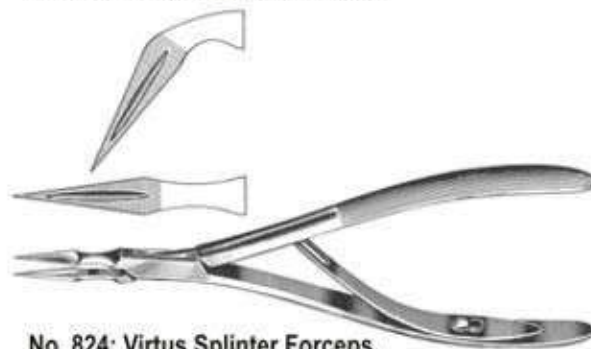
No. 824: Virtus Splinter Forceps, 6" Straight, Stainless.
